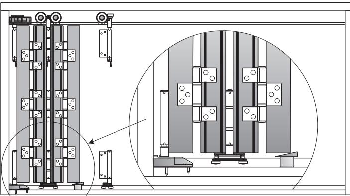
21. ADDING PANELS
