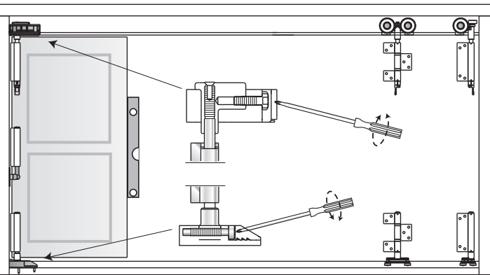
20. PANEL ADJUSTMENT
