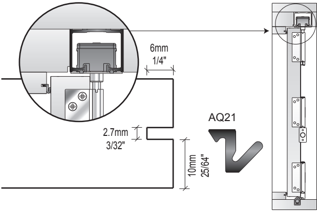
8. PERIMETER SEAL
