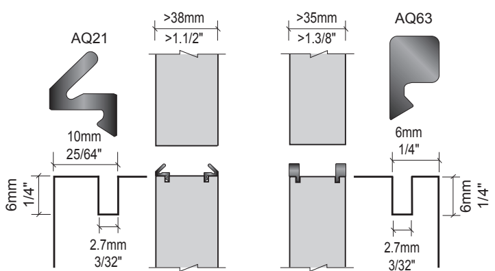
9. PANEL SEALS
