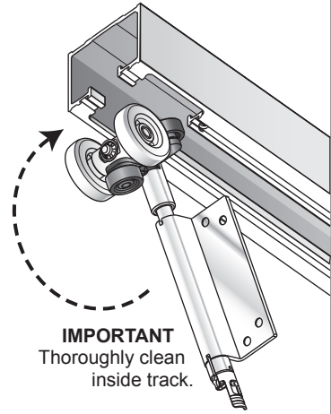
15. INSTALLATION
