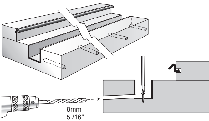
6. CHANNEL FIXING - DRAINAGE
