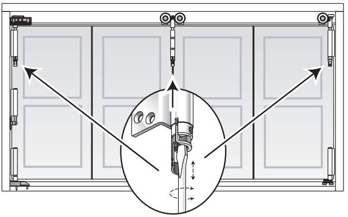
22. FINAL ADJUSTMENT
