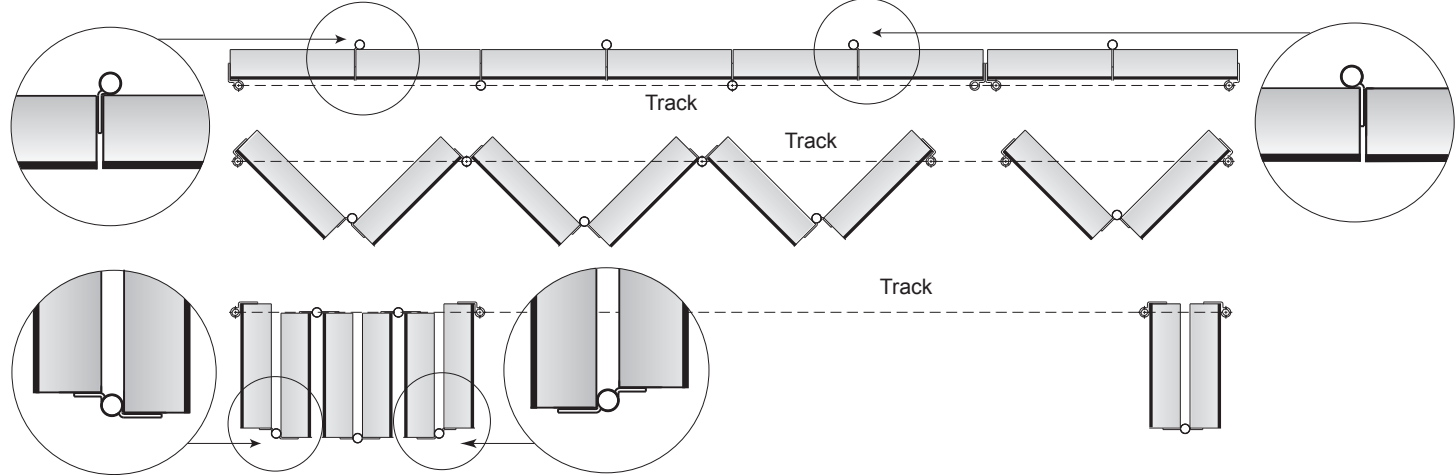
11. PANEL ORIENTATION
