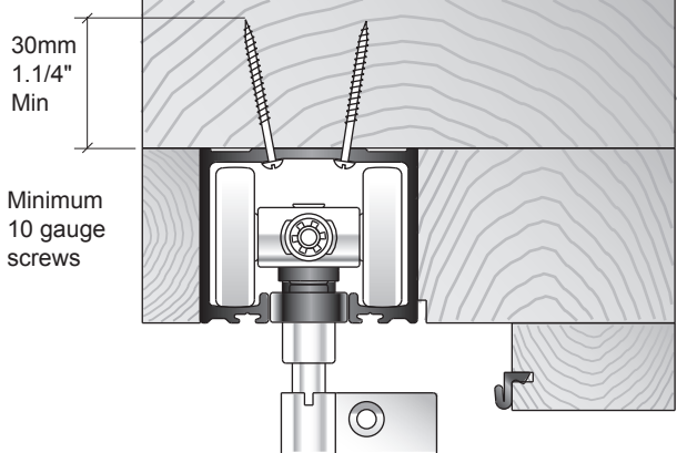
4. TRACK FIXING & CARRIER CLEARANCE
