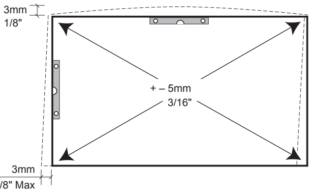
1. INSTALL FRAME
